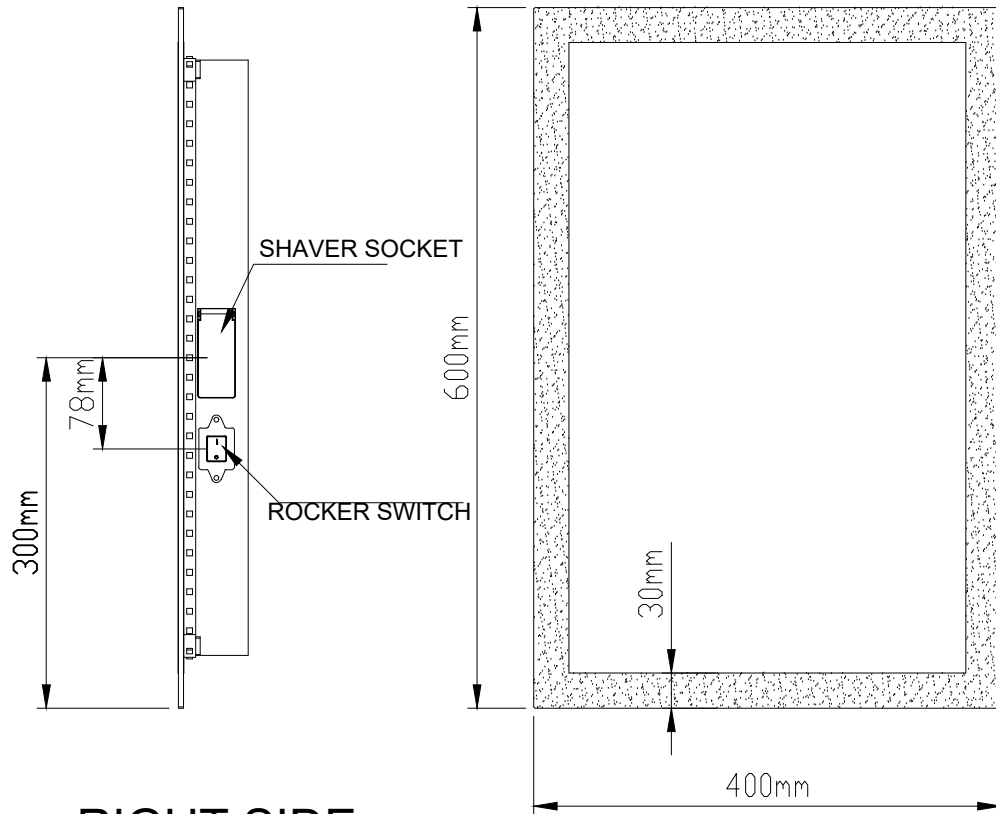
RIGHT SIDE
