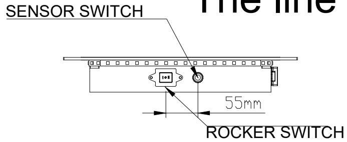
BOTTOM VIEW
