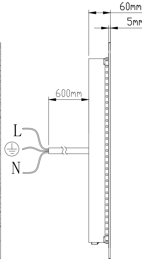
BOTTOM VIEW
