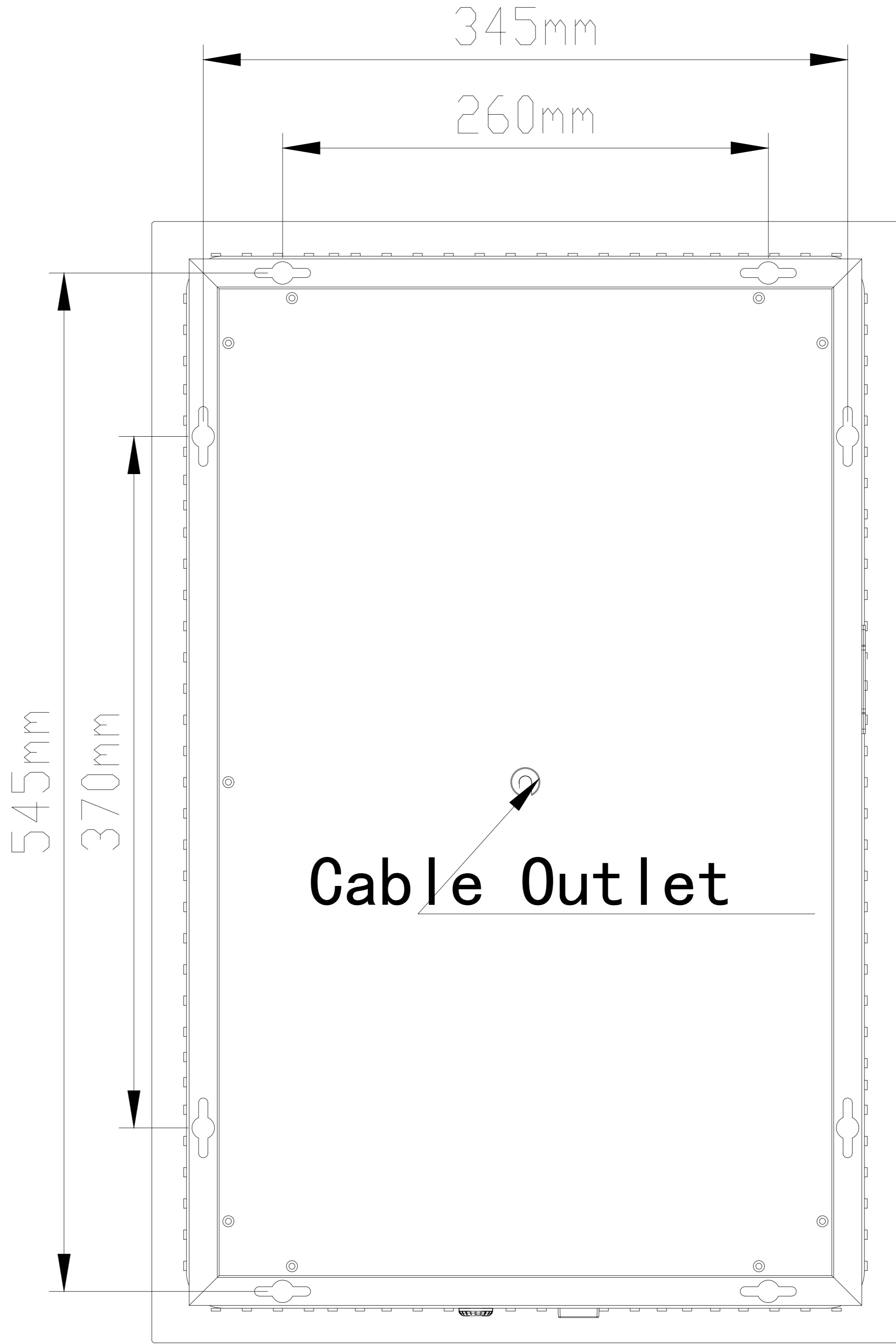
REAR VIEW
